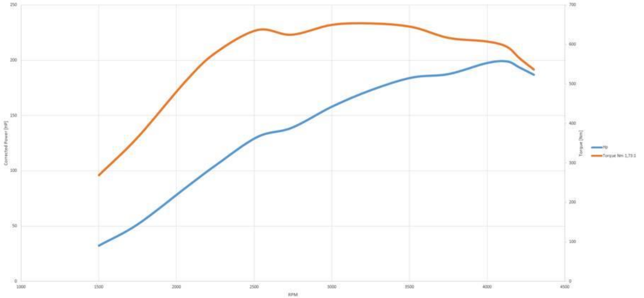
OXE-200 Torque & Power Curve (1,73:1)
